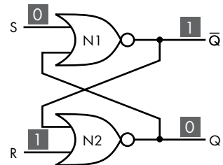
Figure 6-3: SR latch, initial state
