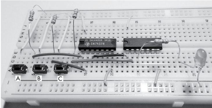
Figure 4-24: Breadboard implementation of (A \text{ OR } B) \text{ AND } C
