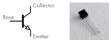
Figure 4-5: The symbol for (left) and photo of (right) an NPN transistor
