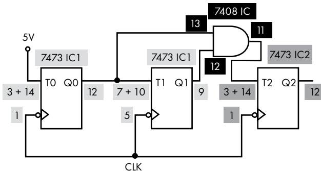
Figure 6-29: A 3-bit counter built from T flip-flops, pin numbers shown
