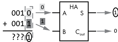
Figure 5-8: Half adder in action
