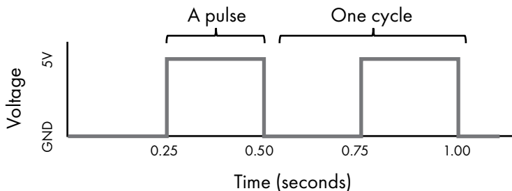
Figure 6-11: A 2Hz clock signal
